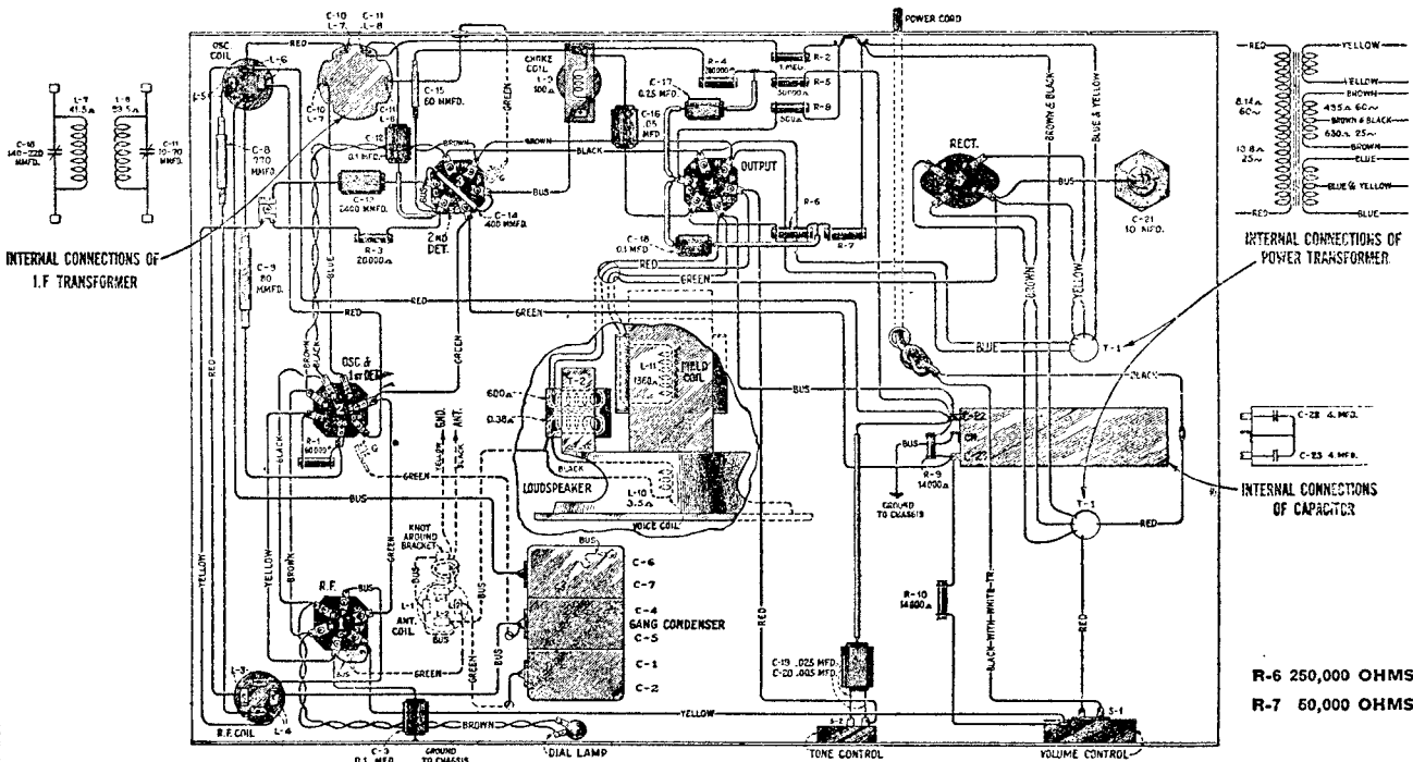
Wiring Diagram
